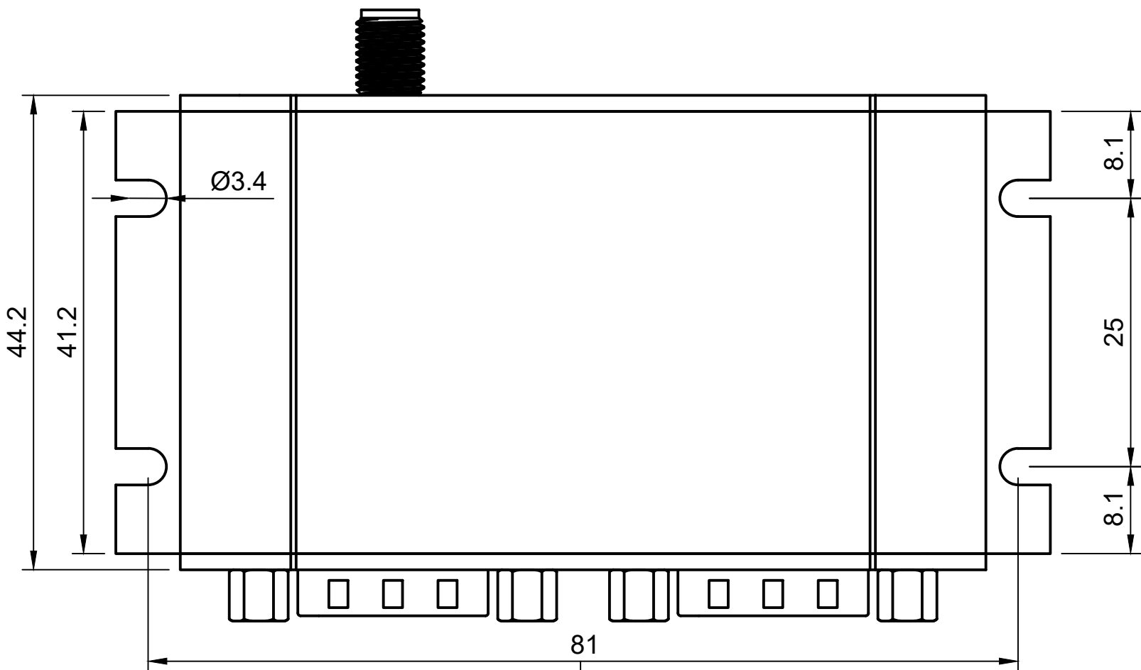
Top view
