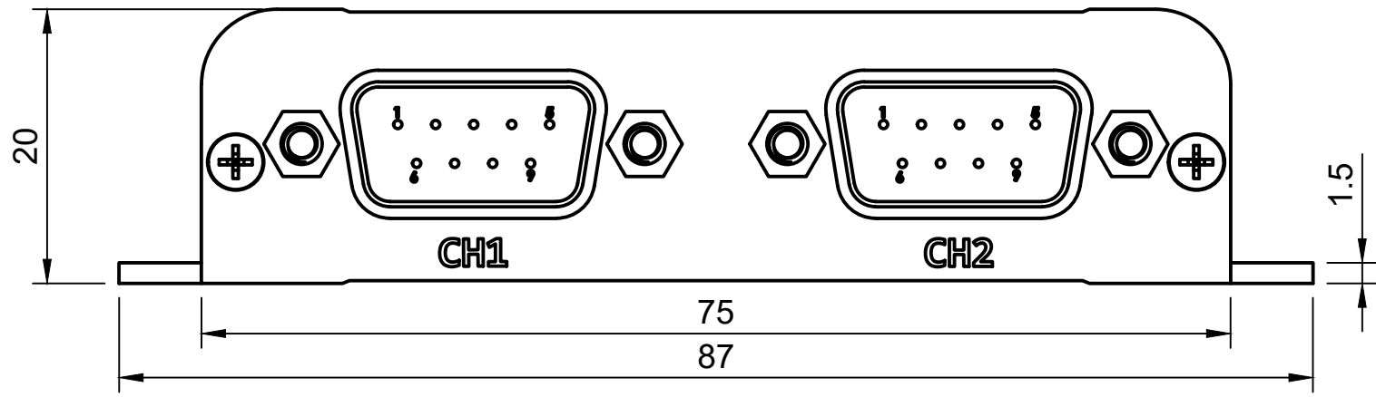
Front view
